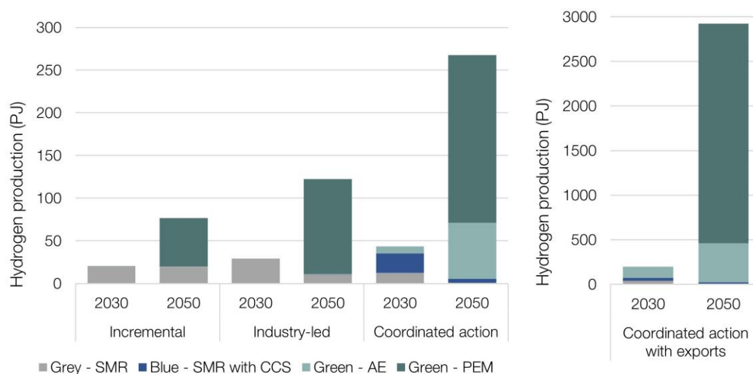
Figure 34: Hydrogen production
