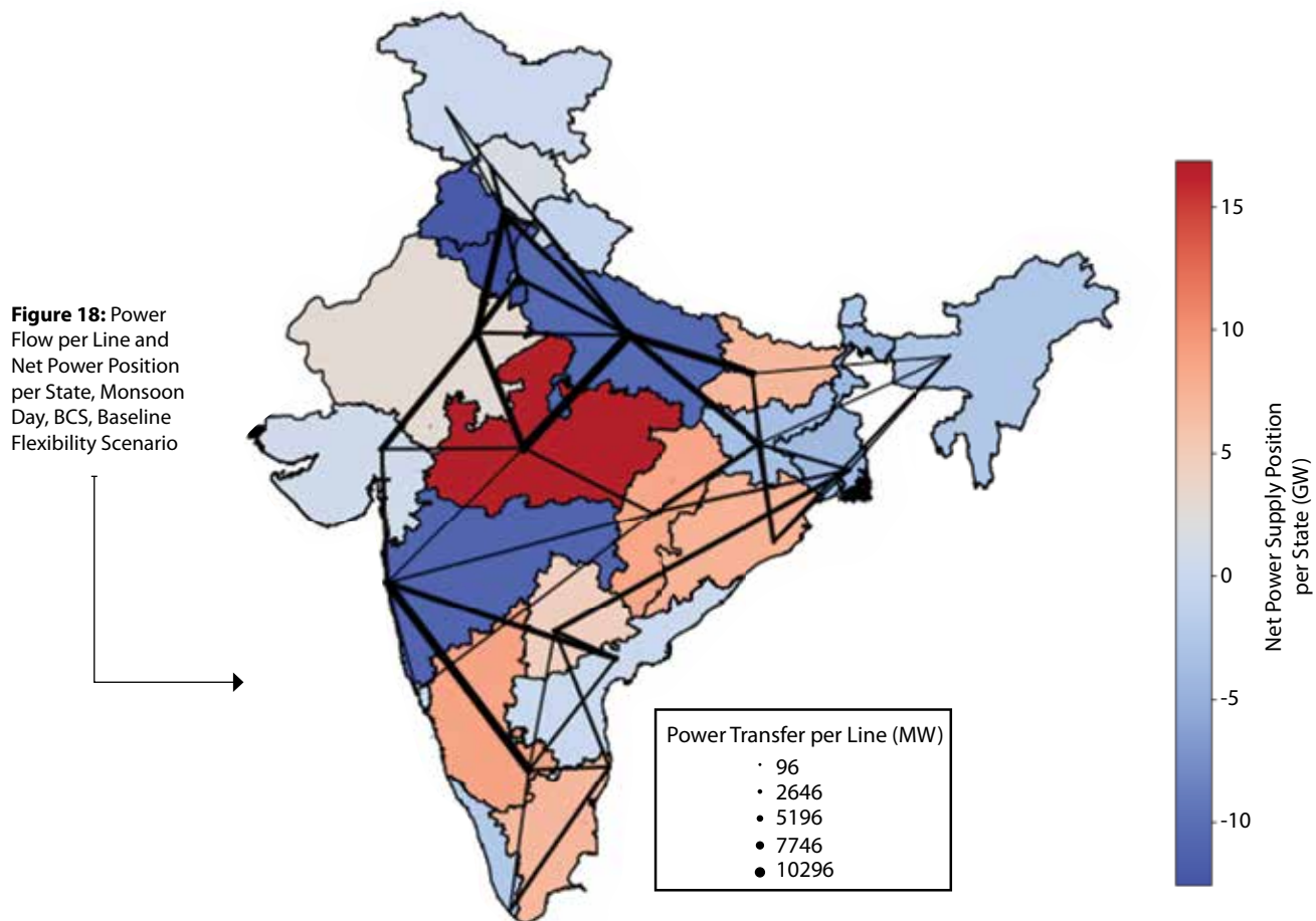
Power Flow per Line and Net Power Position per State at 1 pm on 24-06-2030
