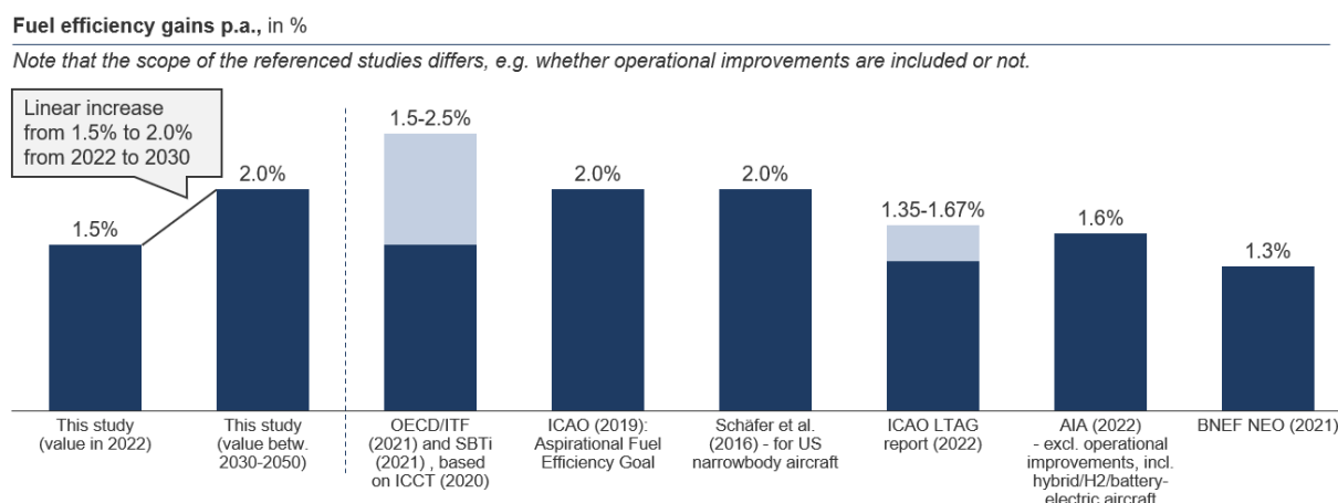
Exhibit 1: Fuel efficiency gains assumed in this study, compared with assumptions of other reports. 6,8-15
