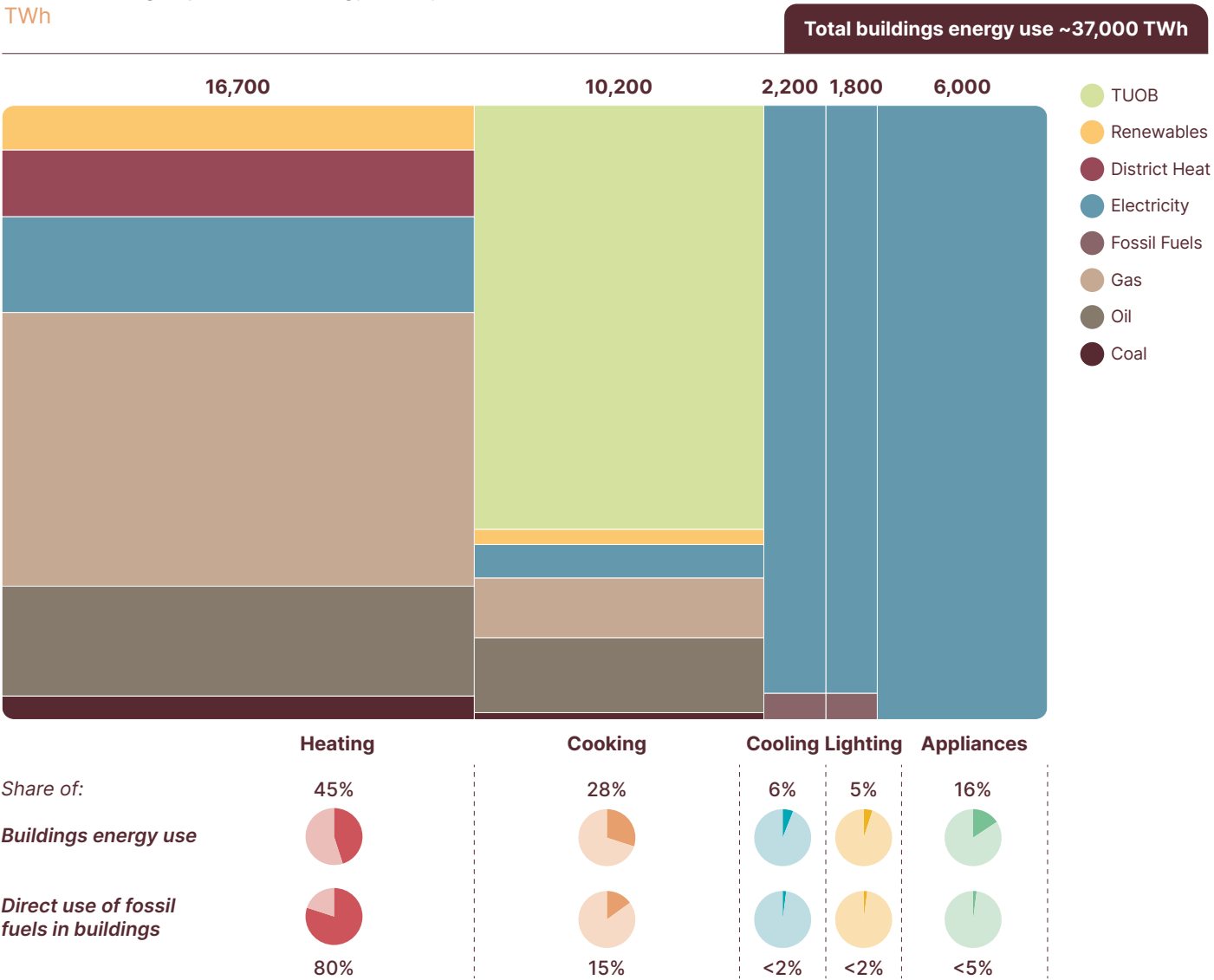
Global buildings operational energy use by end-use and fuel, 2022
