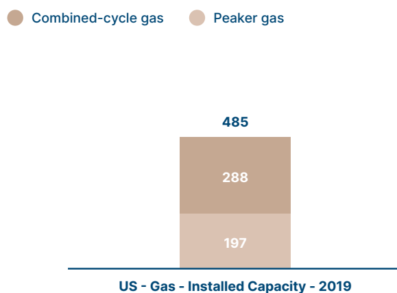
US gas capacity by technology, GW
