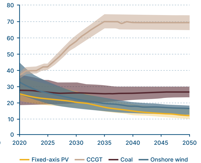
Levelised cost of new PV and onshore wind vs. running costs of existing coal and gas: India $/MWh, (2019 real)
