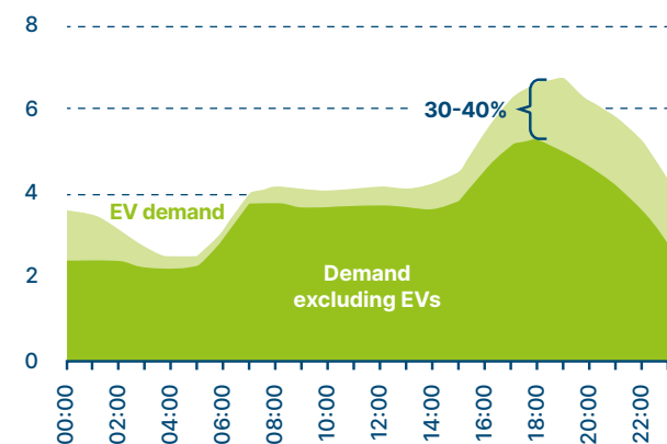
EV impact on typical 11kW feeder in the U.K., with 50% of houses owning an EV GW
