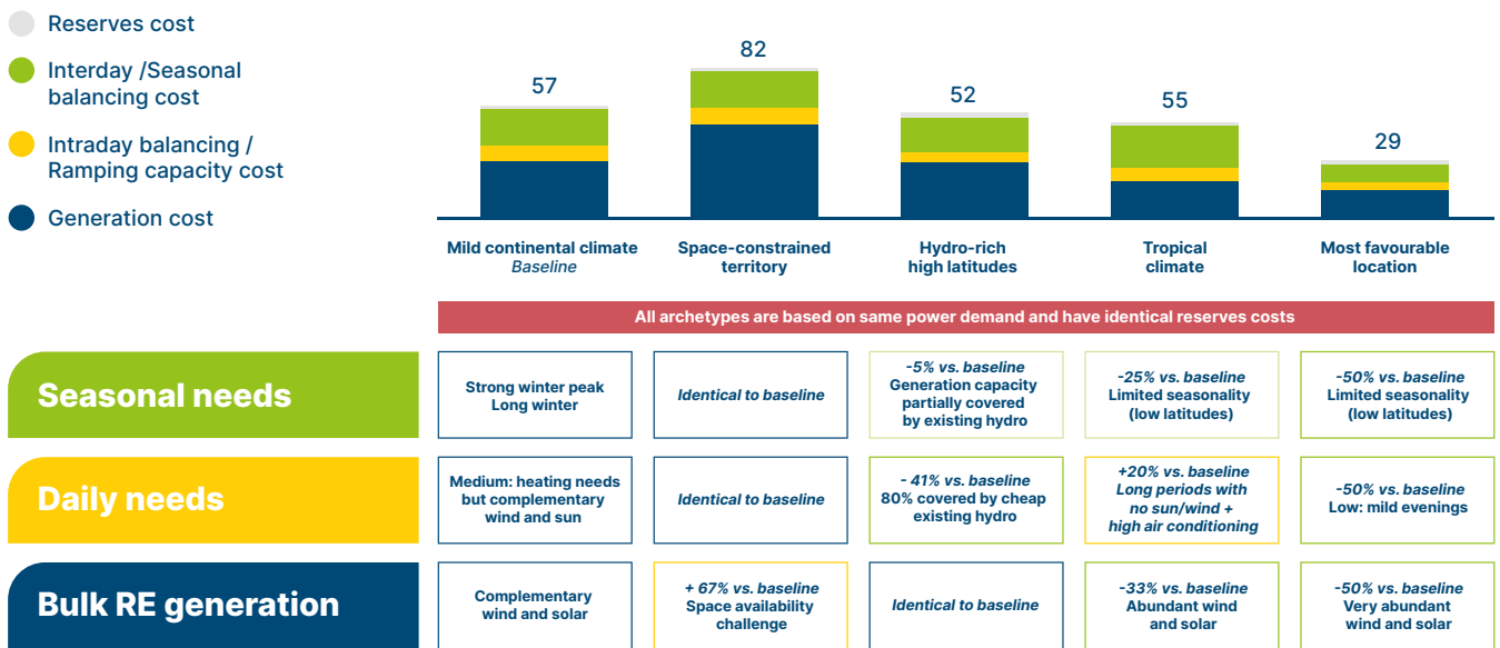
Maximum all-in cost of power generation in a near-total-variable-renewable power system by 2035 $/MWh, breakdown by flexibility services
