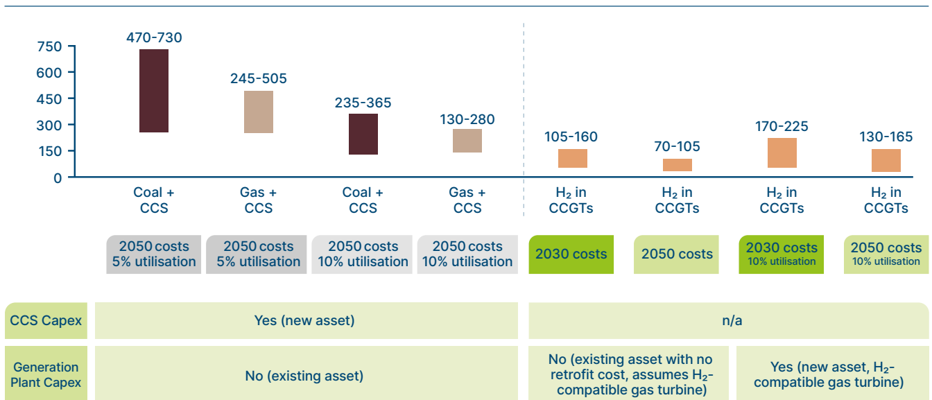
Indicative levelised cost of electricity (LCOE), $/MWh
