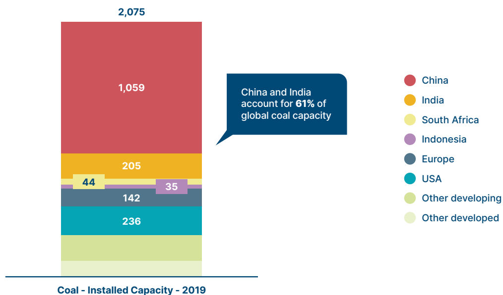
Global coal capacity by region, GW
