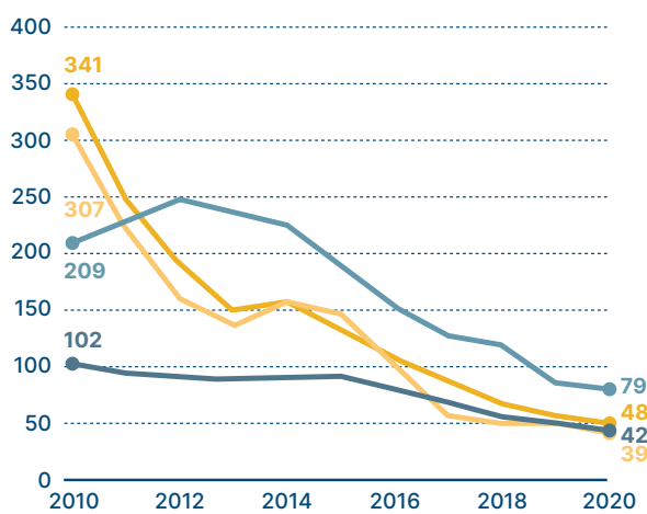
PV and wind LCOE global benchmarks LCOE, $/MWh, 2019 real
