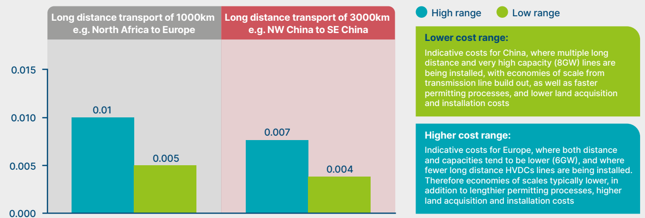
All-in indicative cost of HVDC electricity transmission across distances 2 $/(kWh*1000 km)
