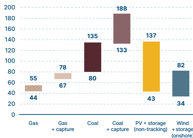
Comparison of US LCOEs in 2023 $/MWh, (2018 real)
