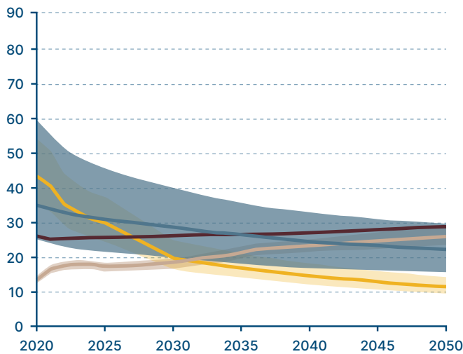
Levelised cost of new PV and onshore wind vs. running costs of existing coal and gas: US $/MWh, (2019 real)
