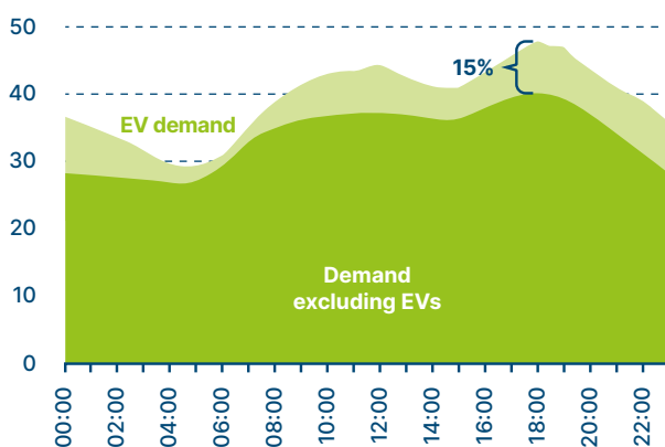
EV impact on U.K. national power demand at 50% EV adoption GW
