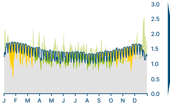
German yearly power demand profile in a near 100% VRE system, Daily TWh
