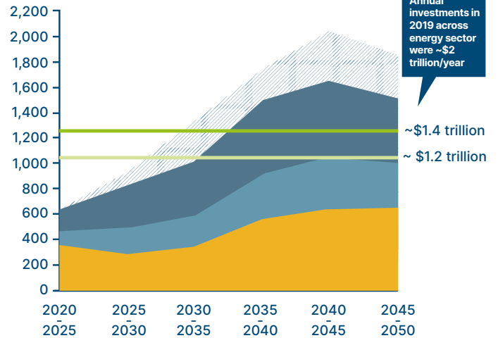
Average annual capital investments in generation (wind and solar) $ billion per year, average across 5-year period
