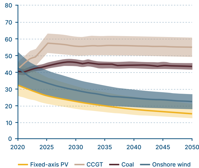
Levelised cost of new PV and onshore wind vs. running costs of existing coal and gas: China $/MWh, (2019 real)
