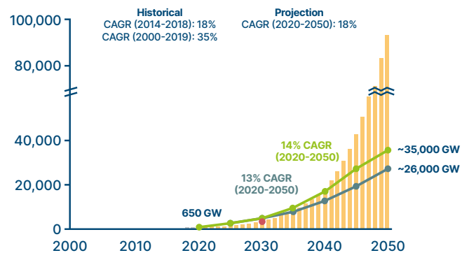
Solar – cumulative installed capacity GW
