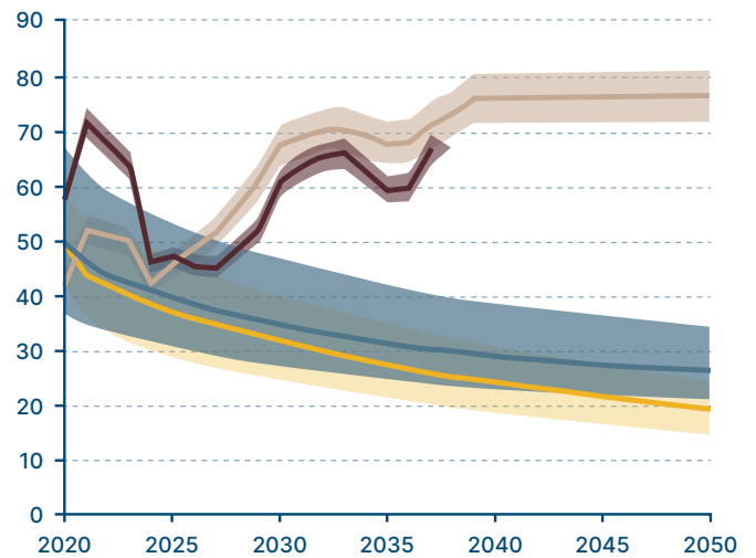
Levelised cost of new PV and onshore wind vs. running costs of existing coal and gas: Germany $/MWh, (2019 real)
