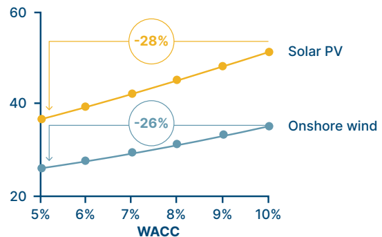
Illustrative LCOE, WACC for US wind and solar 1 , $/MWh, %
