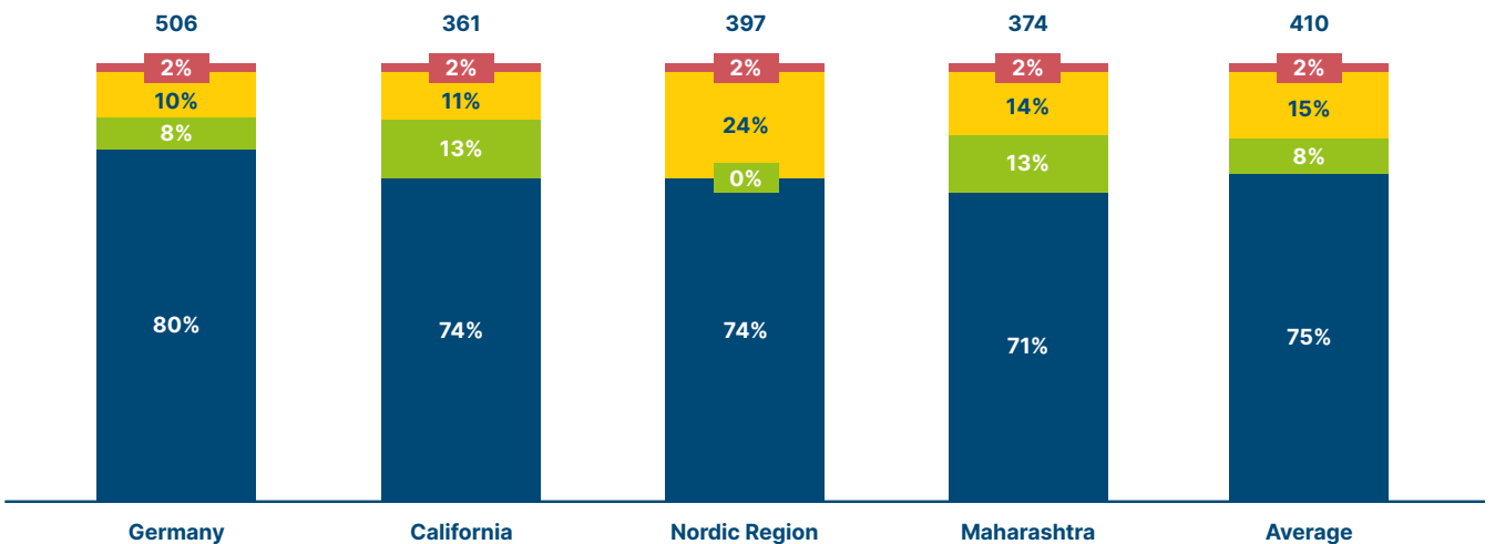
Balancing variability across markets in a near 100% VRE system
