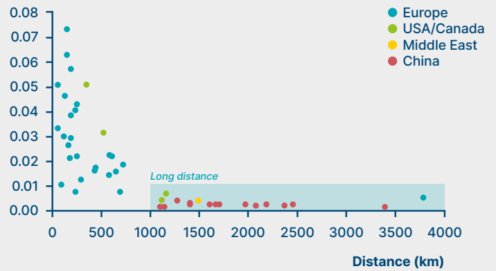
HVDC Capex cost of electricity transport (projects in development, excludes financing cost) 1 $/(kWh*1000 km)
