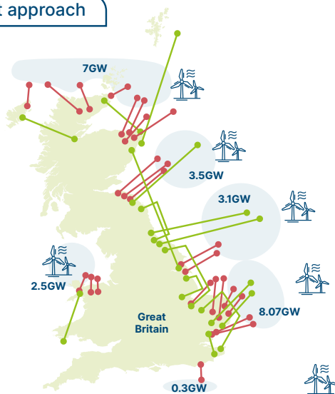
UK offshore wind network development models
