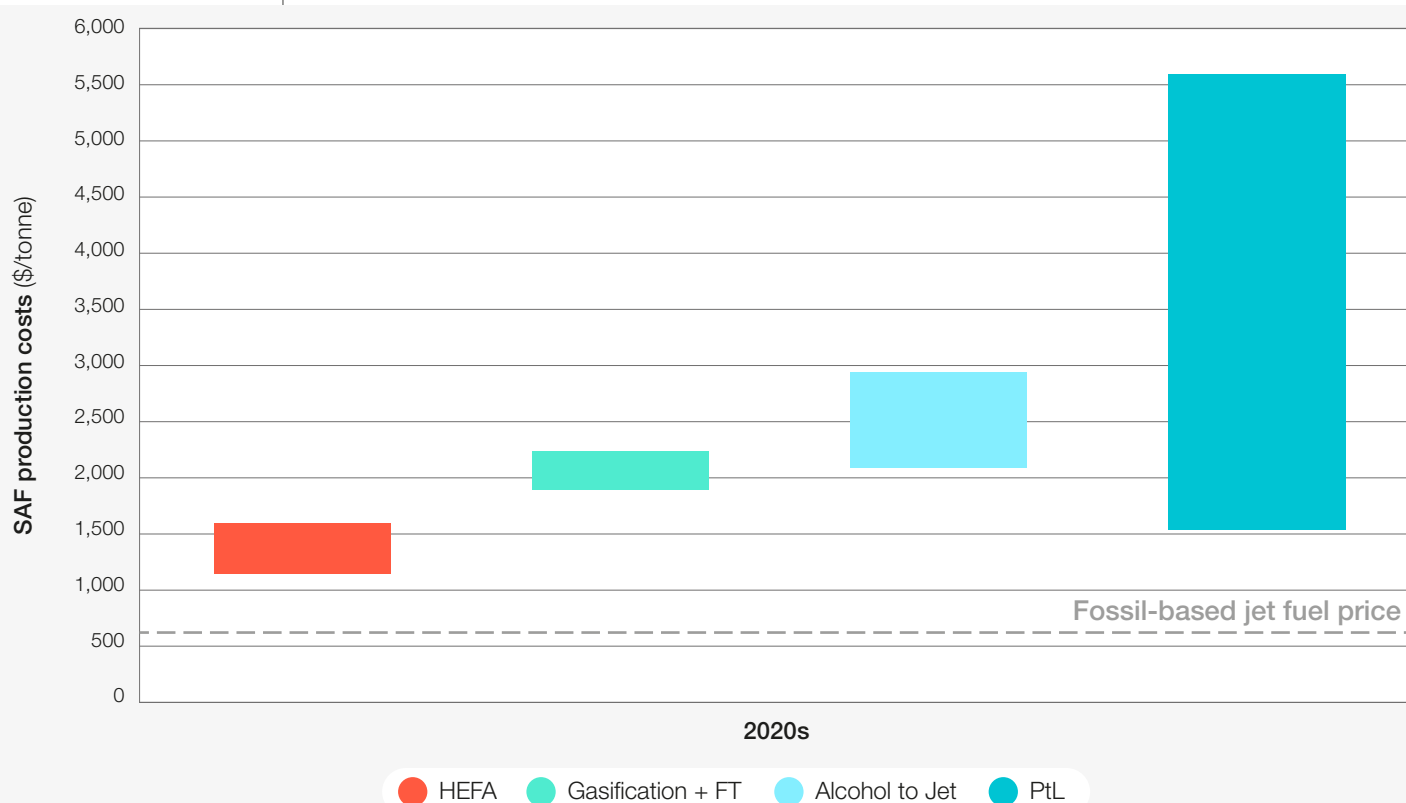
FIGURE 3 Indicative SAF costs by production pathway
