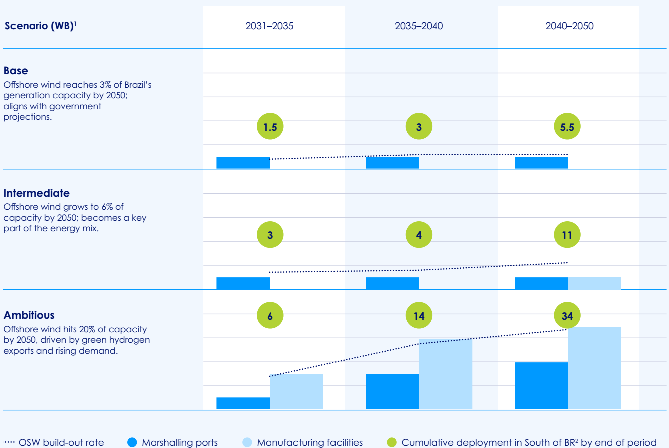
FIGURE 11 SCENARIOS FOR OFFSHORE WIND DEPLOYMENT AND ASSOCIATED PORTS IN THE SOUTH OF BRAZIL
