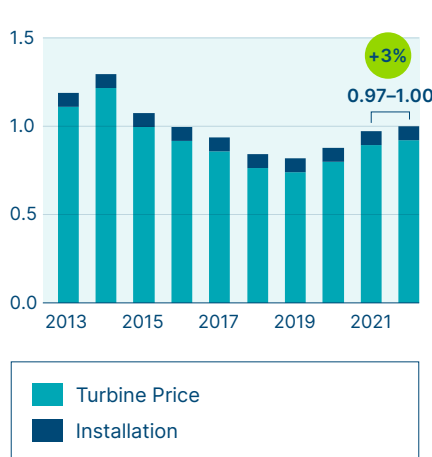
Wind turbine price by signing date 2022 $m/MW
