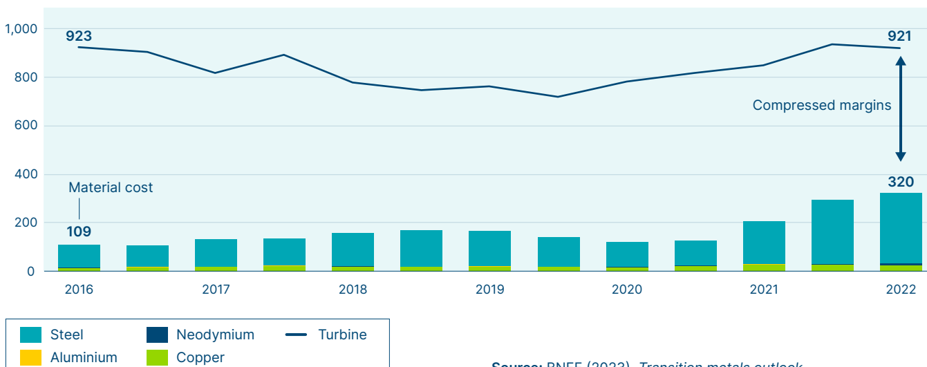
Metal and total wind turbine price Thousand $/MW
