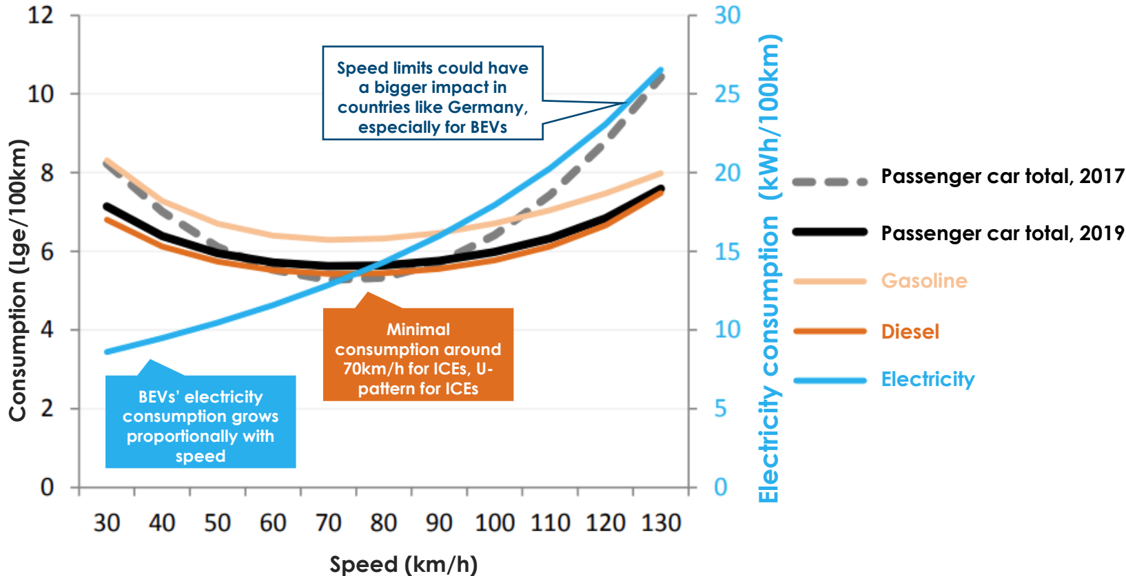
Relationship between speed and energy consumption for passenger vehicles Km/h, Lge/100km, kWh/100km
