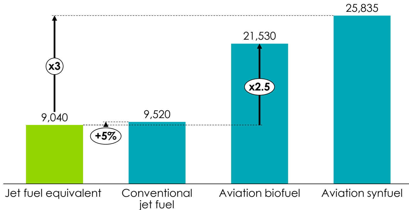
Final versus primary energy demand to produce all of aviation Jet fuel demand in 2050 TWh
